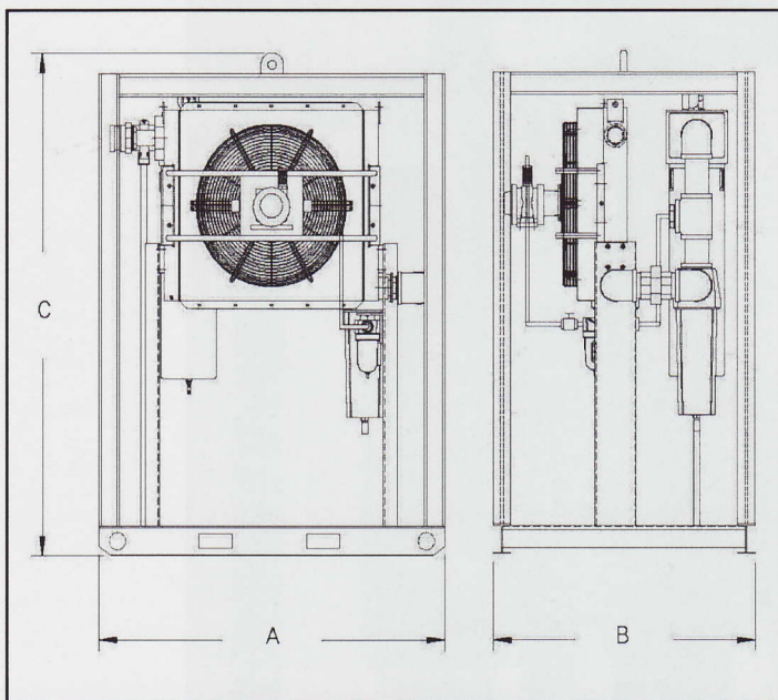
SPAF Series Aftercooler/Filter Separator
