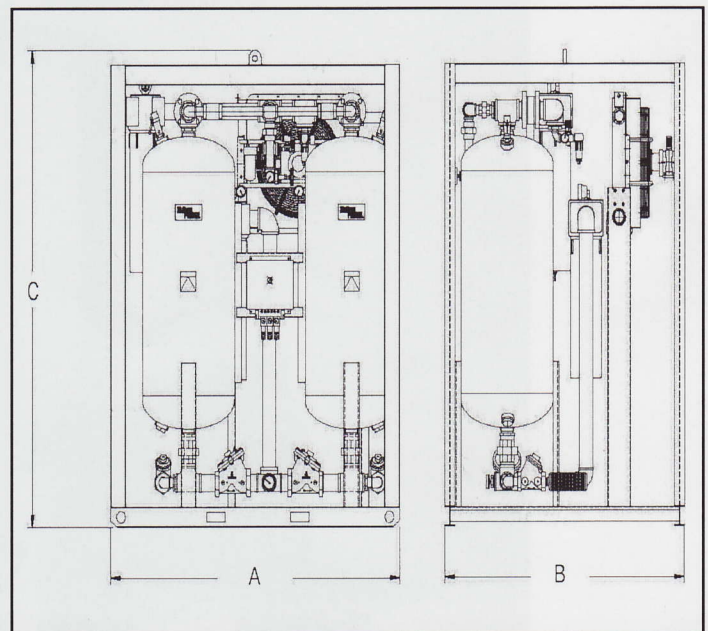
SPS Series Dryer/Aftercooler/Filter Separator
